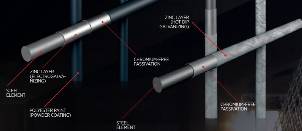
Mesh panel protected by: electrogalvanizing and polyester coating
