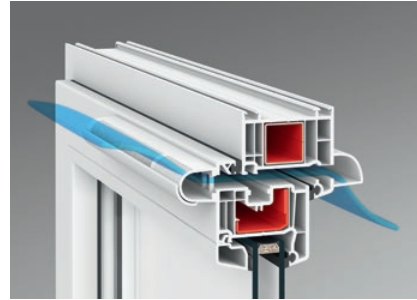
Aereco EMM pressure sensitive air inlet
