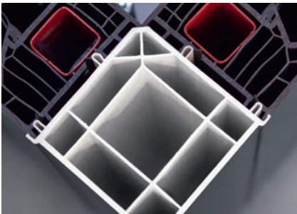
Coupling profiles
