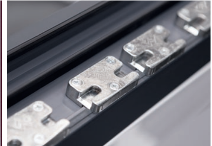
Anti-burglary striker plate in the RU leaf
