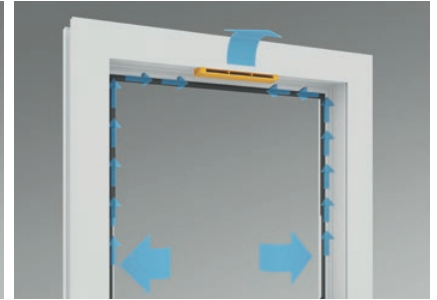
MACO Vent window rebate valve
