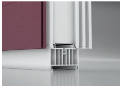
Transport and installation bar
