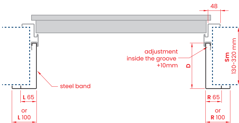
HORIZONTAL CROSS SECTION
