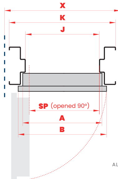
HORIZONTAL CROSS SECTION
