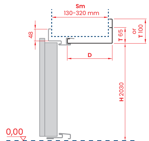
VERTICAL CROSS SECTION
