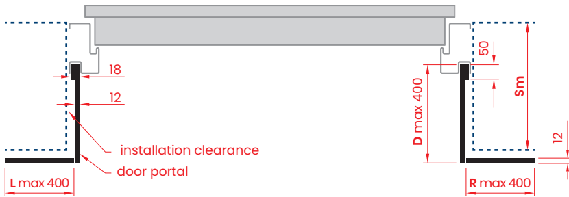
HORIZONTAL CROSS SECTION
