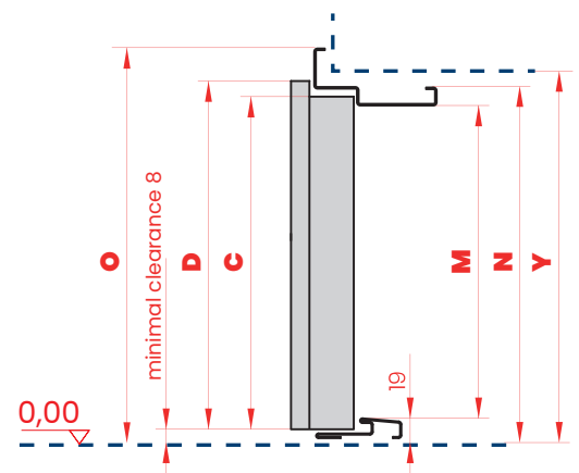
VERTICAL CROSS SECTION
