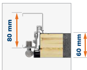
PERFOTHERM 60 door frame
